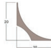
Cove former (4011)
