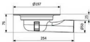
Minimax Compact Drain (090G)
