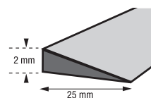
Capping strip (0490)
